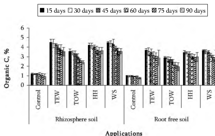
Figure 2 - Changes of total organic carbon in rhizosphere and root free soil. Vertical bars are standard errors. HH = Hazelnut husk, WS = Wheat straw, TOW = Tobacco production waste, TEW = Tea production waste
