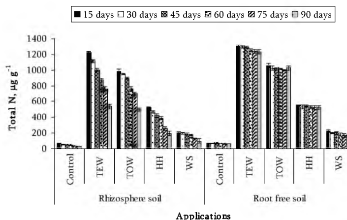
Figure 1 - Changes of total nitrogen in rhizosphere and root free soil. Vertical bars are standard errors. HH = Hazelnut husk, WS = Wheat straw, TOW = Tobacco production waste, TEW = Tea production waste
