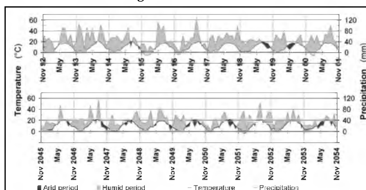
Figure 1 - Time series of precipitation and temperature for station Müncheberg (Top: Initial Situation 2000, Bottom: Scenario 2050 [8])
